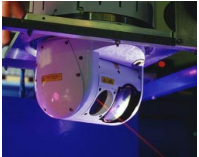
The state of the art in infrared countermeasures are directed infrared jammers. These use gimballed infrared trackers and either a modulated laser or flashlamp to jam the MANPADS reticle seeker. Depicted is the Northrop-Grumman/Marconi DIRCM turret. A typical installation would use a Doppler radar, infrared or ultraviolet Missile Approach Warning System to cue the turret which uses its integral tracker to point the modulated light source at the incoming missile (Northrop Grumman).
